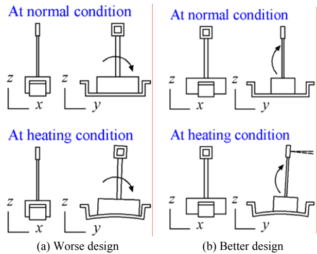
Fig. 10 Two types of holders and mirrors
