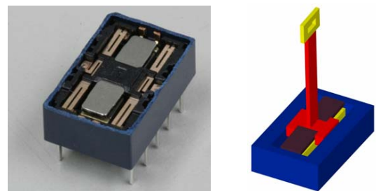
(a) Relay (b) Actuator Fig. 2 The actuator for the optical switch
